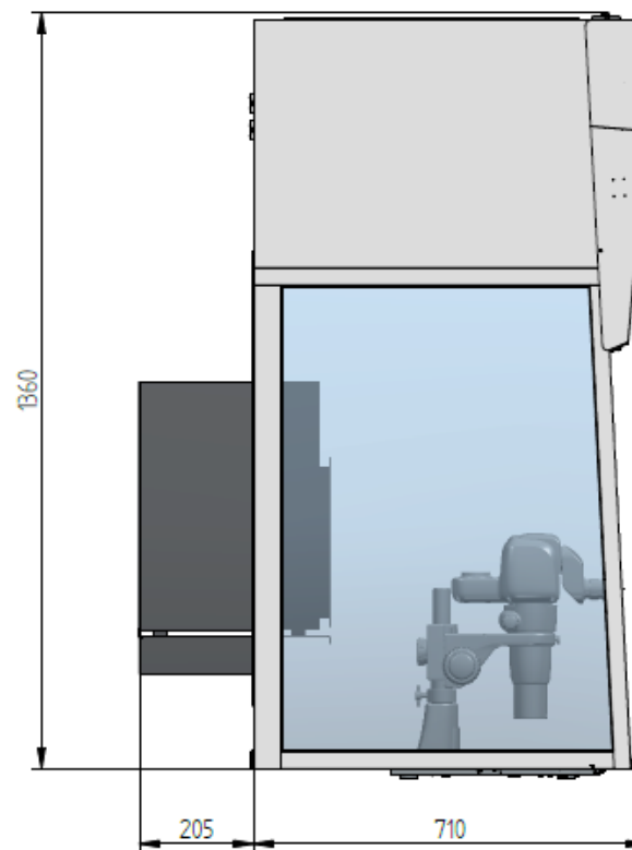
FBB-12 with heating pad (600 × 290 mm), microscope-ready, and integrated CO2 incubator
