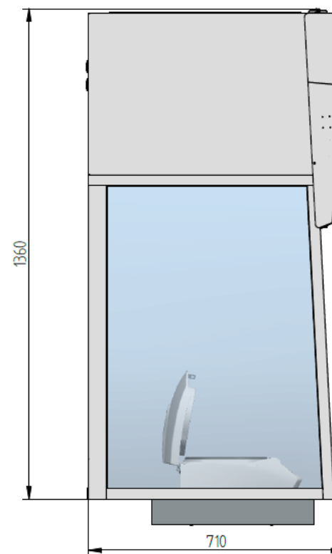
FBB-12 with heating pad (600 × 290 mm) and integrated cenrifuge EBA 200
