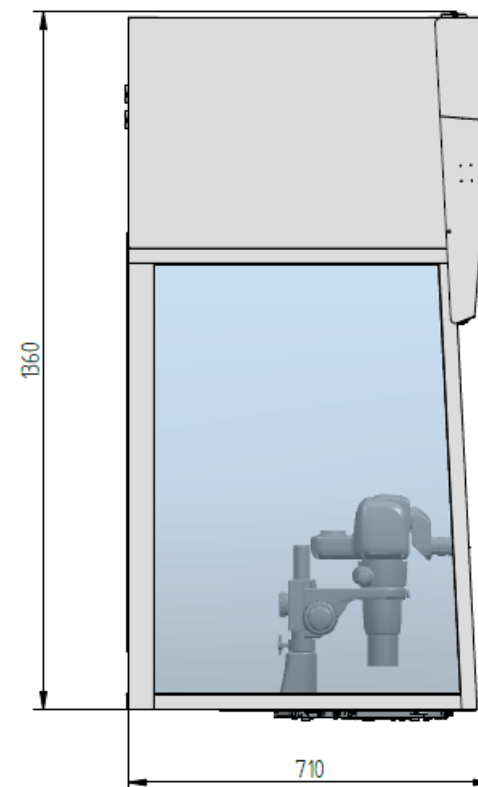
Laminar airflow workstation FBB-12
