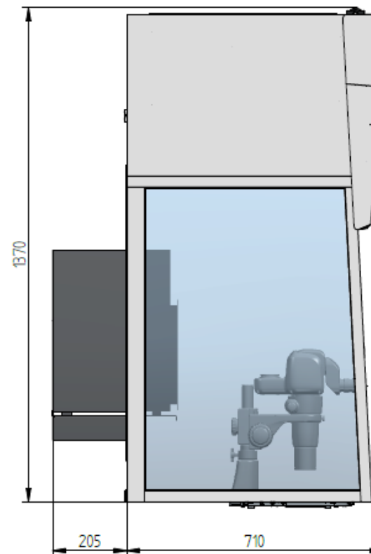
Laminar airflow workstation FBB-12
